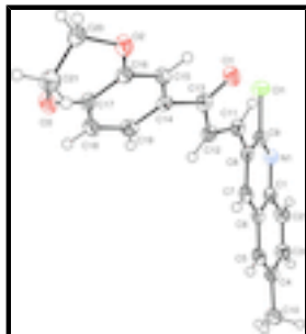
Fig. 1. ORTEP-3 (Farrugia, 1997) drawing of (I) with displacement ellipsoids plotted at 50% probability level.
